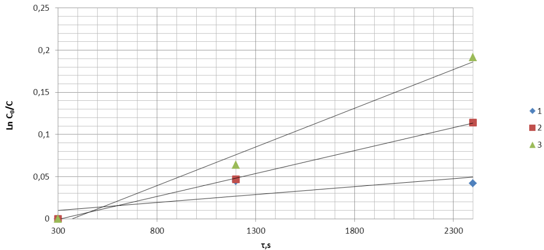
Fig. 7 Kinetic curves of polymerization process of the fraction 140-190°C for the first order reaction (1 – 20°C , 2 – 40°C, 3 – 60°C).
