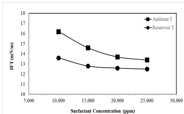
Figure 4. Interfacial tension versus PKO surfactant concentration under different temperature conditions
